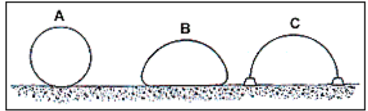
Figure 20. The three common types of metal culverts are classified by shape: (A) corrugated round, (B) corrugated pipe-arch, and (C) structural plate-arch. (Redrawn from Furniss et al. 1991, p. 316)
