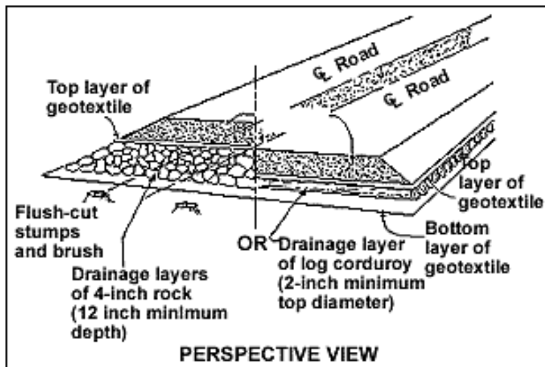
Figure 22. Proper roadbed construction in peat wetlands allows free water flow. (Redrawn and adapted from Minnesota Department of Natural Resources 1995, p. 50)
