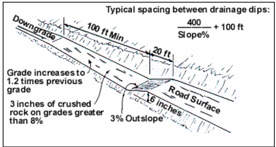
Figure 11. Drainage dips are broad structures used on roads with grades of 10 percent or less.
