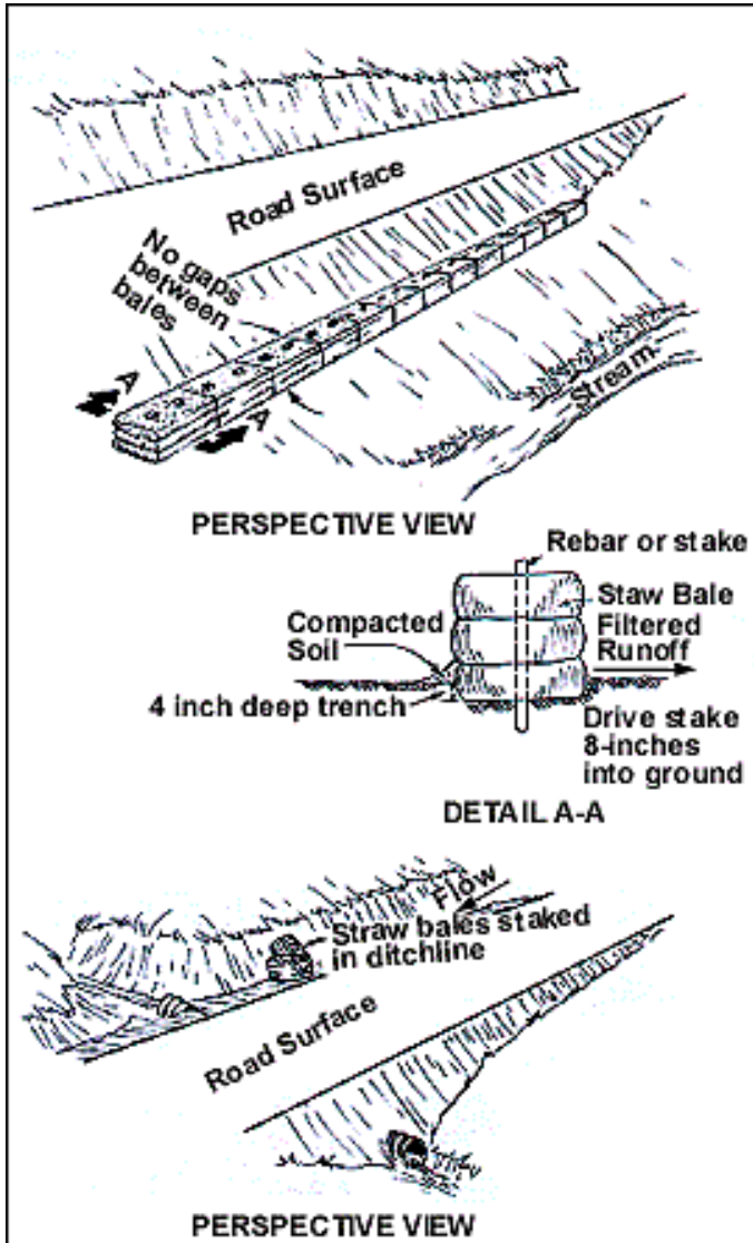
Figure 18. Use stabilization practices on soil exposed at stream crossings during
