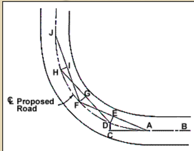
Figure 3. The stick method of creating a horizontal curve is suited to use on difficult terrain. (Redrawn from Figure 2.4-2, Darrach et al. 1981)
