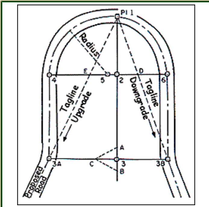
Figure 4. A switchback is needed when a straight road would exceed maximum acceptable grade. (Redrawn and adapted from Figure 2.4-3, Darrach et al. 1981)
