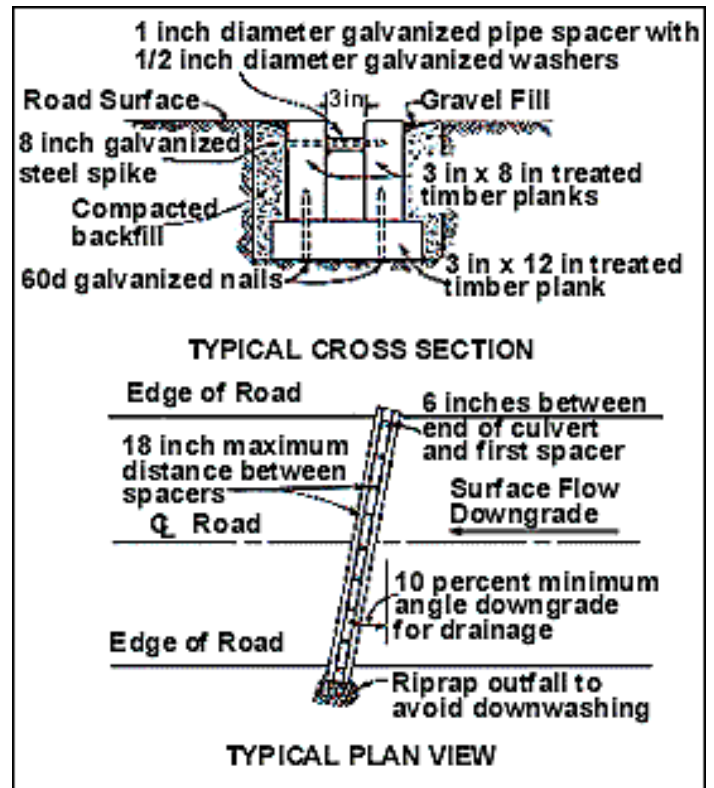
Figure 13. For an open-top culvert to function properly, careful installation and regular maintenance are necessary.
