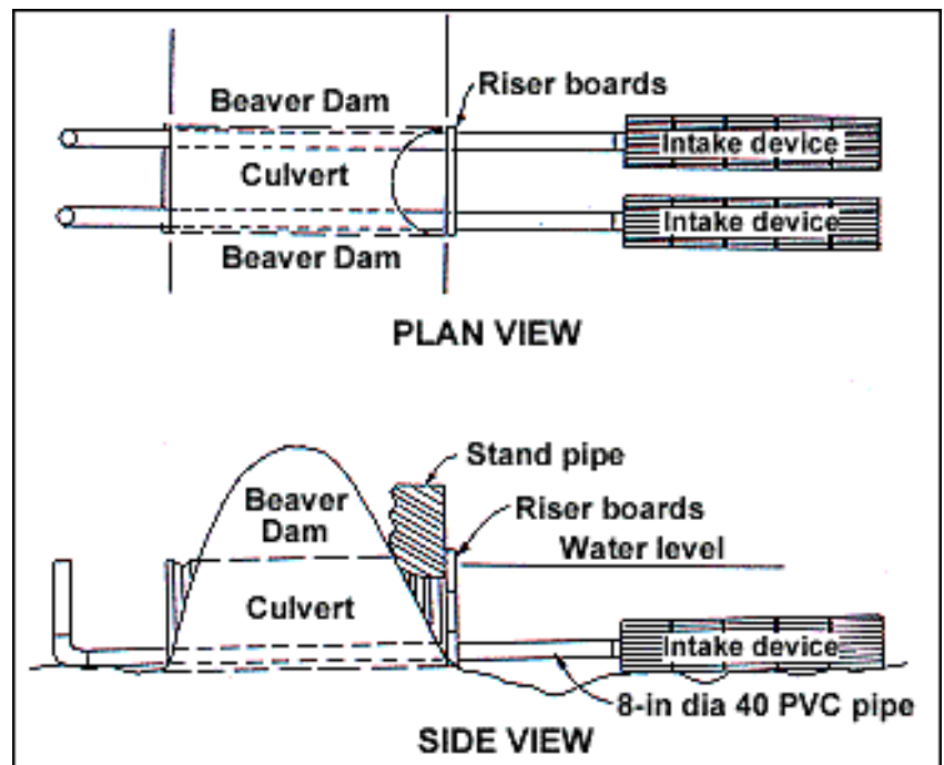
Figure 27. The Clemson Beaver Pond Leveler helps solve plugging of road culverts, as well as filling of stand pipes and culverts used as water control structures. (Redrawn from Wood et al. 1994, p. 3)
