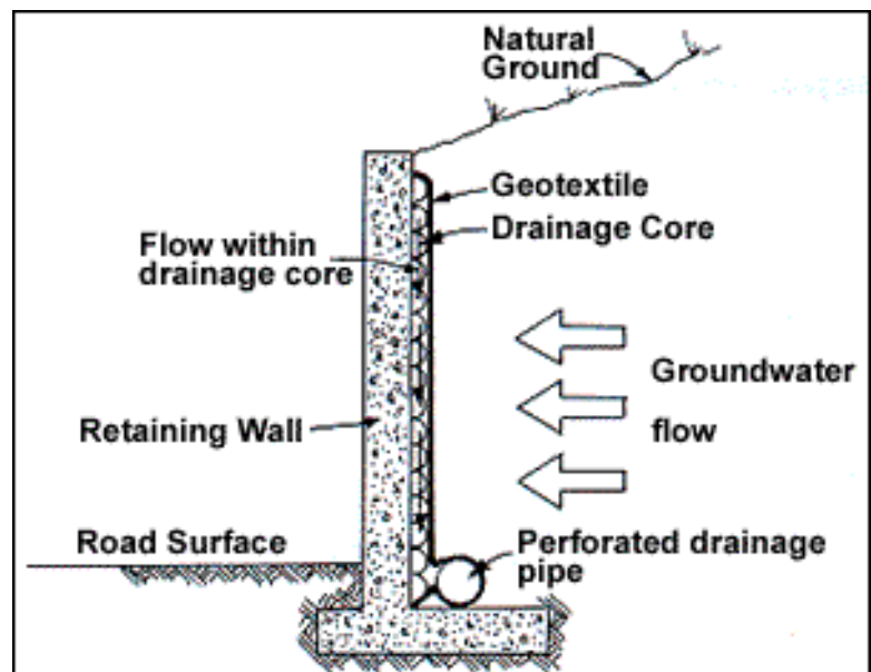
Figure 32. Composite geotextile material allows water flow within the plane of the material, rather than across it, such as behind a retaining wall. (Redrawn with permission from Figure 10, Amoco Fabrics and Fibers Company 1994a, p. 6)
