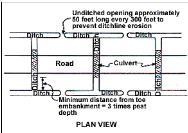
Figure 23. Adequate cross-drainage throughout the road length is essential in deep peat wetlands. (Redrawn from Minnesota Department of Natural Resources 1995, p. 51)
