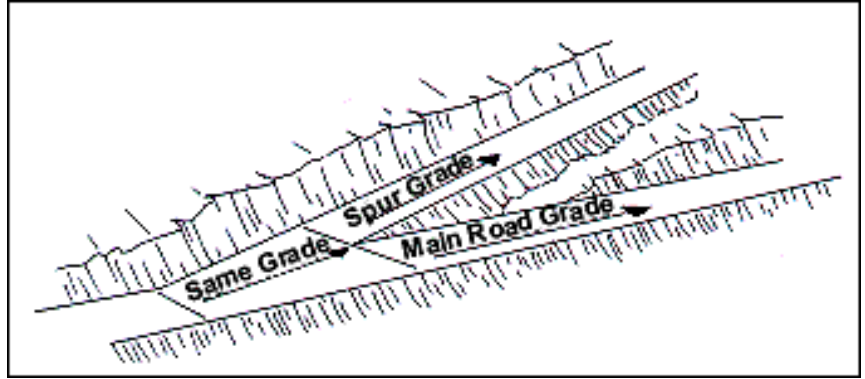
Figure 5. A main road and spur must have the same grade for a distance equal to at least the sum of half the width of each. (Redrawn and adapted from Figure 2.4-7, Darrach et al. 1981)
