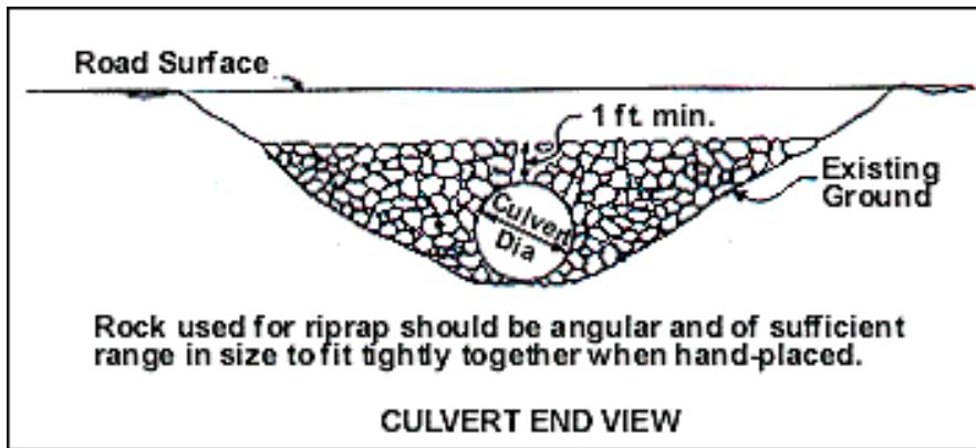
Figure 19. Install riprap to prevent erosion at the inlet to a culvert pipe.
