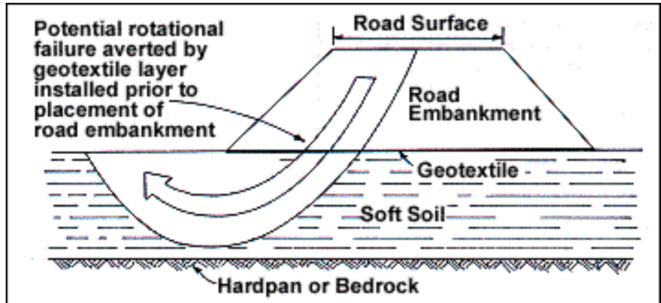
Figure 31. Geotextile material under the roadbed reinforces soft soil and preserves the road embankment. (Redrawn with permission from Figure 8, Amoco Fabrics and Fibers Company 1994a, p. 5)
