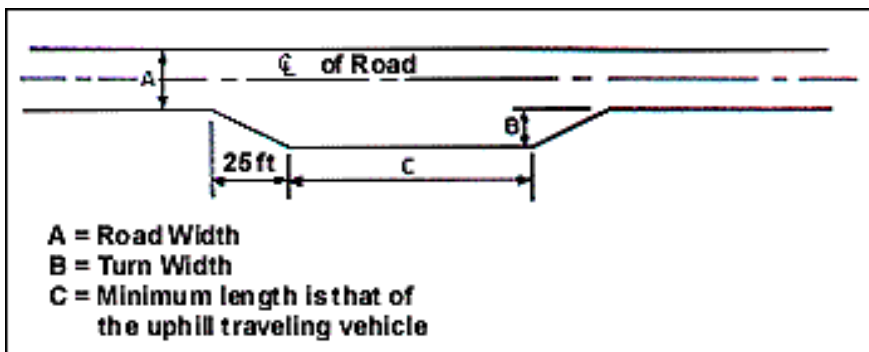
Figure 7. A turnout should be at least 10 feet wide, to allow two trucks to pass safely. (Redrawn from Figure 2.4-10, Darrach et al. 1981)
