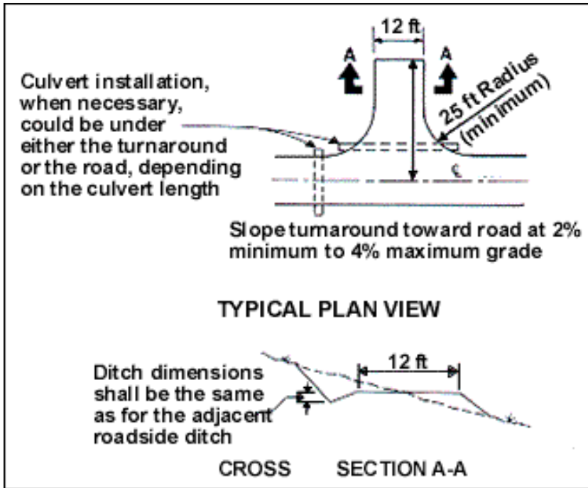
Figure 8. Turnaround design should consider drainage.
