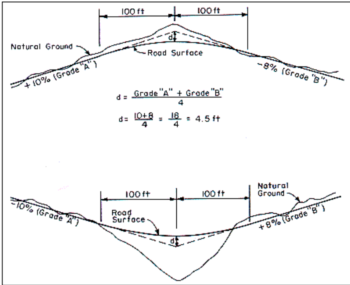
Figure 6. A vertical cut provides a smooth transition on a crest (top), and a vertical fill provides a smooth transition on a sag (bottom). (Redrawn from Figures 2.4-8 and 2.4-9, Darrach et al. 1981)
