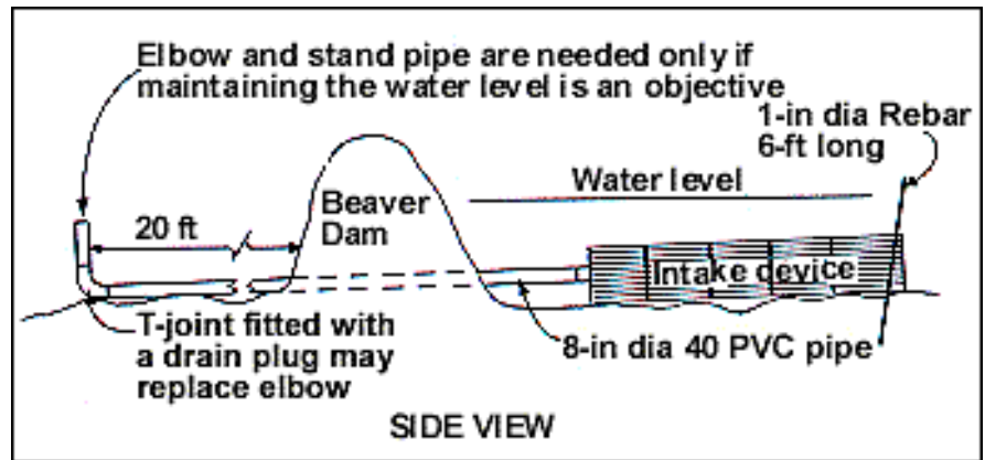
Figure 26. The Clemson Beaver Pond Leveler is a low-cost, low-maintenance solution. (Redrawn from Wood et al. 1994, p. 2)
