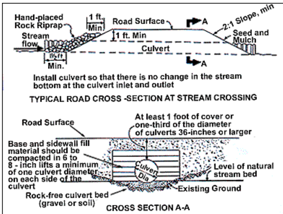
Figure 17. A cross section of a culvert at A-A shows the recommended structure of fill material installed around a culvert pipe. (Redrawn and adapted from Figures 6-5 and 6-6, Wisconsin Department of Natural Resources 1995, p. 26)
