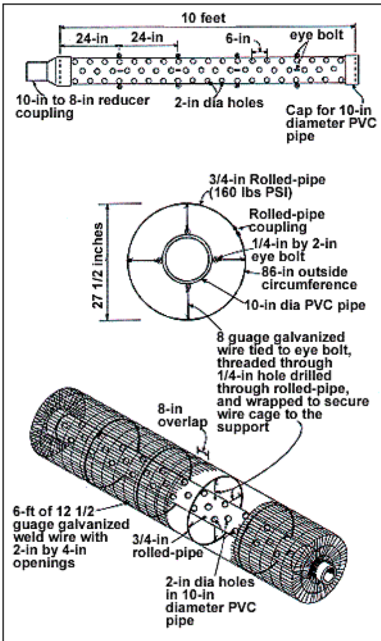
Figure 28. The Clemson Beaver Pond Leveler can easily be constructed of common building materials and installed the same day. (Redrawn from Wood et al. 1994, p. 3-4)
